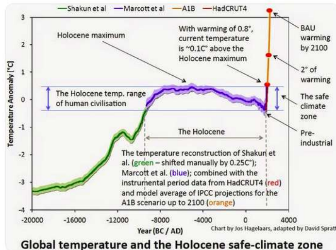
Global temperature and the Holocene safe-climate zone
